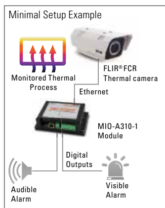
Example 1: Basic Thermal Monitoring with alarms using the MIO-FCR-1
