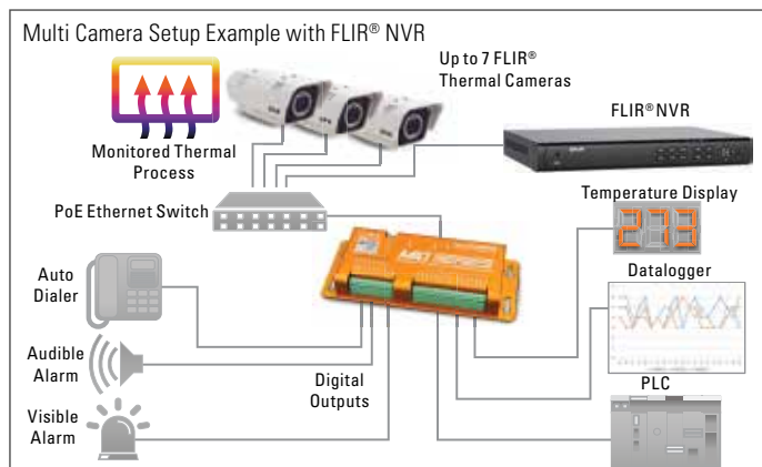
Example 2: Advanced Multi-camera Thermal Monitoring with alarms, automated notification, datalogging, PLC connectivity and real-time video archiving using the MIO-FCR-7
