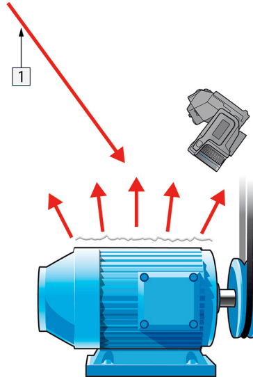
Figure 17.5 Measuring the apparent temperature of the aluminum foil.
