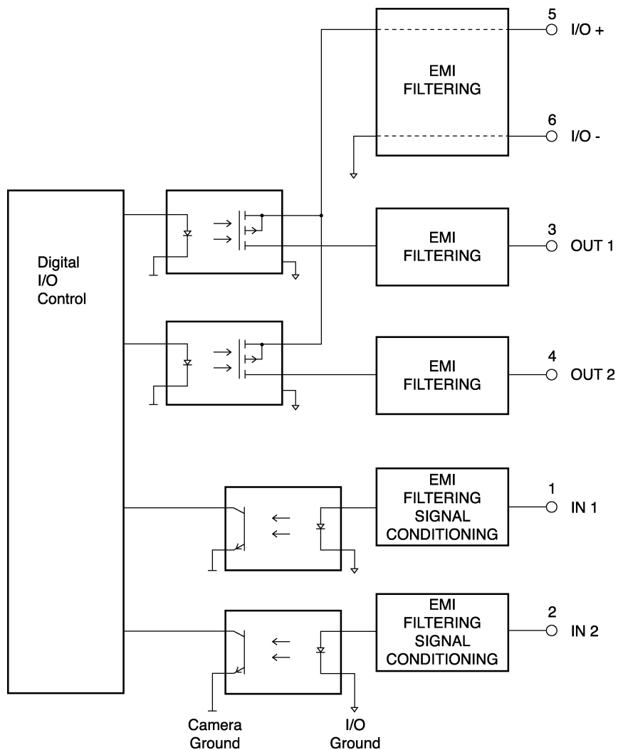
Figure 13.1 Schematic overview of the camera unit digital I/O ports.
