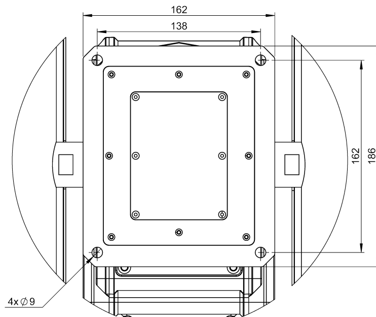
Figure 8.3 FLIR A3xx pt series camera mounting (mm)
